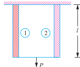
Fig. 4.13. Stresses in composite bars.
