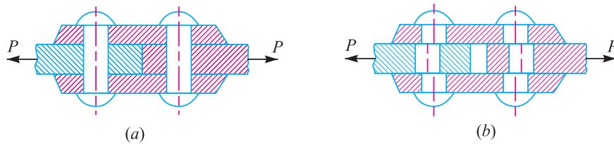
Fig. 4.7. Double shearing of a riveted joint.
