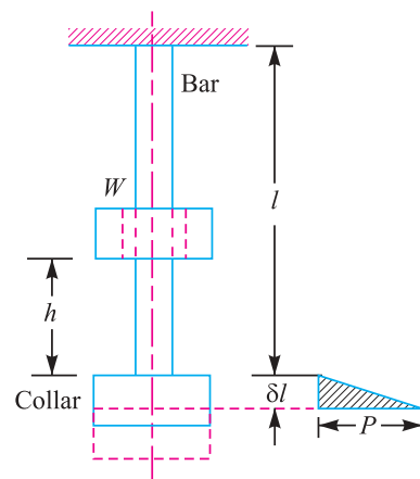
Fig. 4.20. Impact stress.
