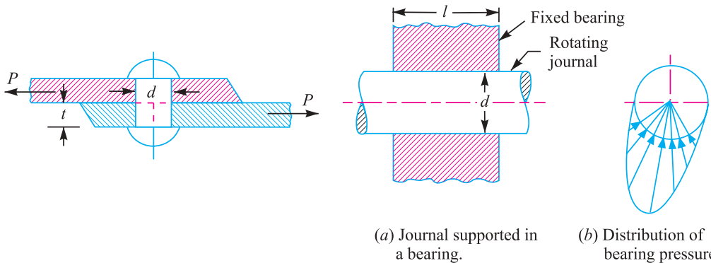
Fig. 4.9. Bearing stress in a riveted joint. Fig. 4.10. Bearing pressure in a journal supported in a bearing.
